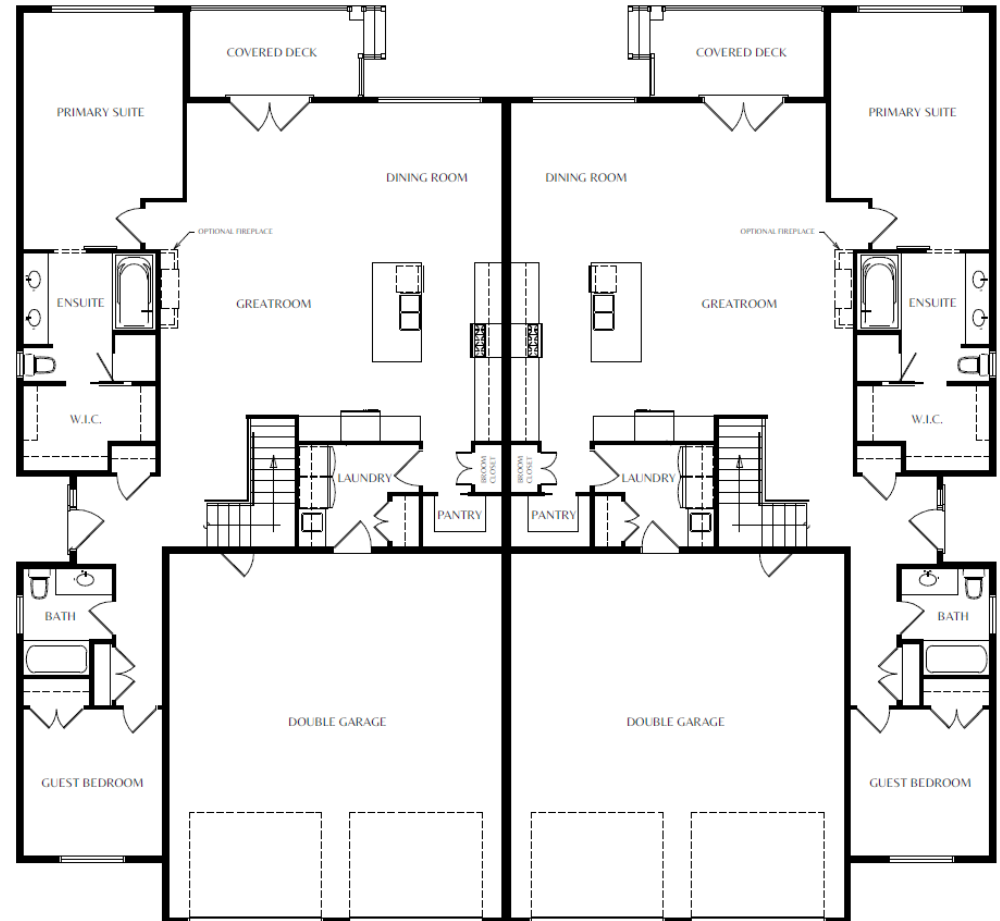
FULL BASEMENT OPTION SHOWING STAIR LOCATION MECHANICAL ROOM LOCATED IN BASEMENT
